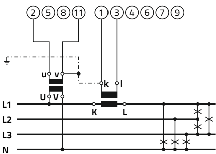
4b - three-phase, four wires, balanced load
