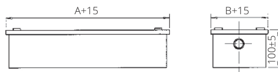
THE CAP FOR KNK9101 (TYPE KNK9151)
