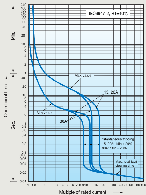
Operating curves
