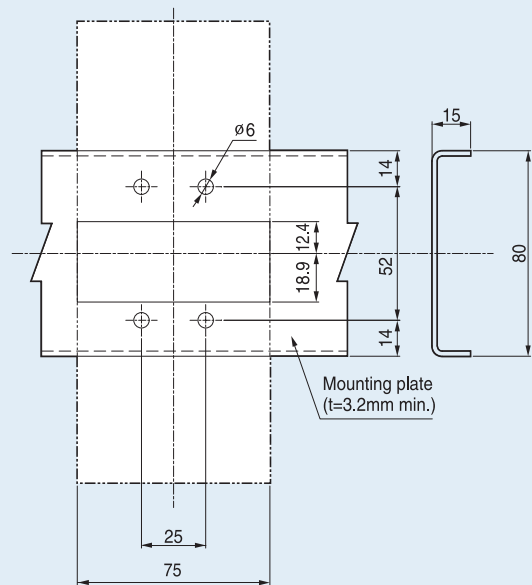
Mounting dimensions
