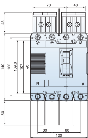
4P (L-type)
