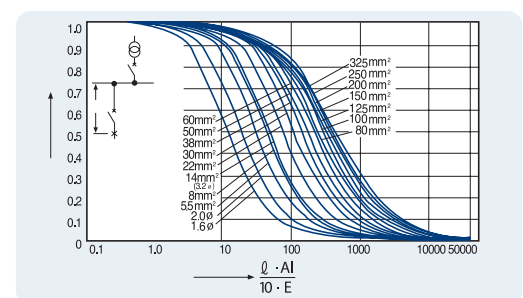
<Fig.10> Decreasing coefficient of general busduct (Cu)
