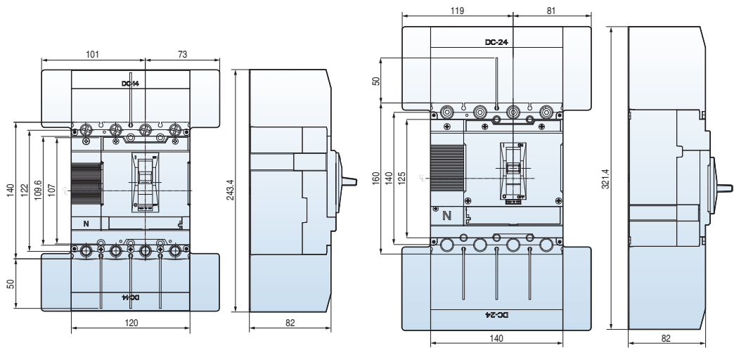
4P (L-type)
