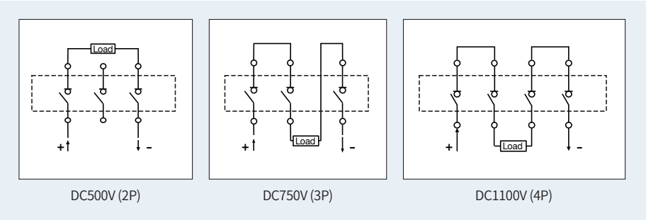
DC Exemplary circuit diagrams
